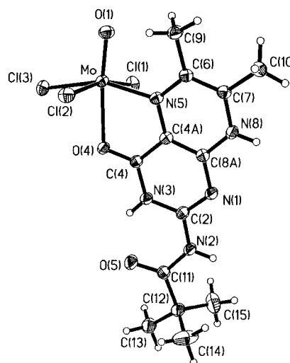
Figure 2. ORTEP diagram of the molecular structure of \text{MoOCl}_3(\text{piv-dmpH}) \cdot \text{EtOEt} ( 2 ) with thermal ellipsoids at 30% probability.
